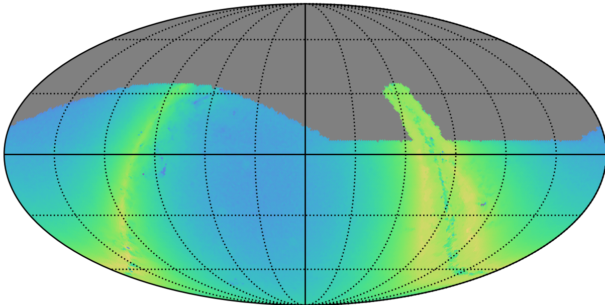
retro_baseline_v2.0_10yrs g: N stars to Precision 0.20
