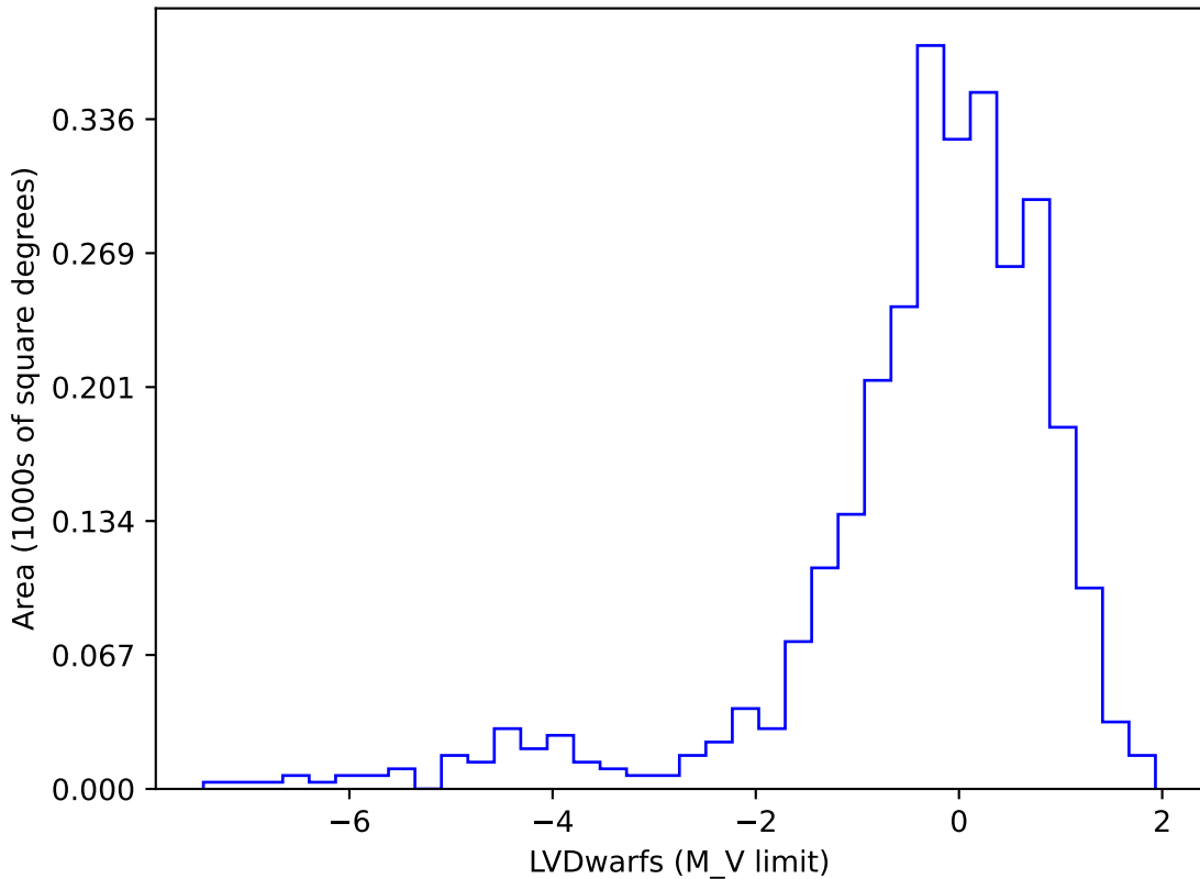
retro_baseline_v2.0_10yrs gi SCP: LVDwarfs
