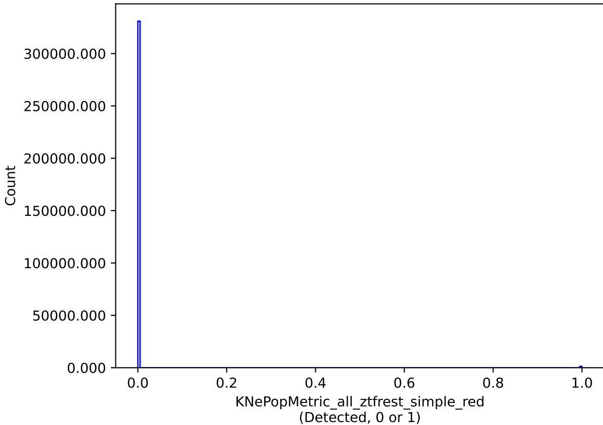
retro_baseline_v2.0_10yrs all models: KNePopMetric_all_ztfrest_simple_red
