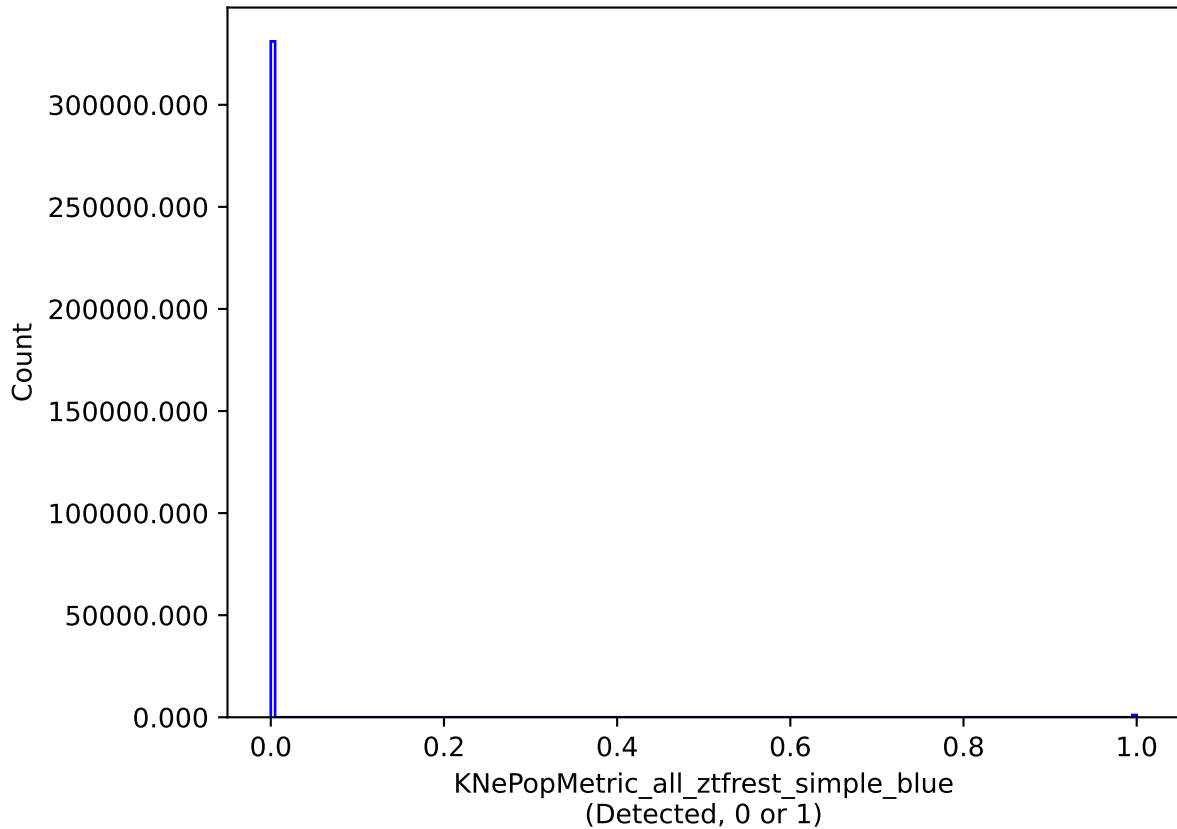
retro_baseline_v2.0_10yrs all models: KNePopMetric_all_ztfrest_simple_blue
