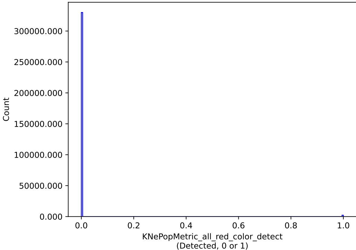
retro_baseline_v2.0_10yrs all models: KNePopMetric_all_red_color_detect
