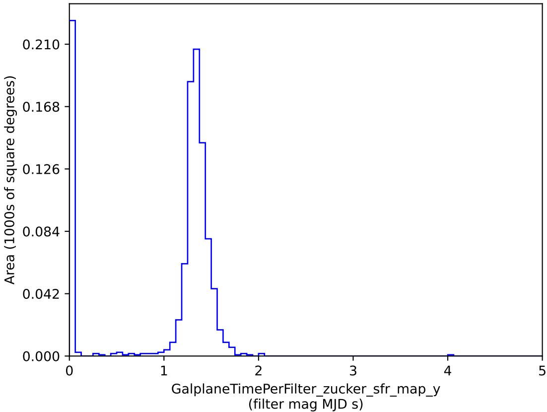
retro_baseline_v2.0_10yrs : GalplaneTimePerFilter_zucker_sfr_map_y
