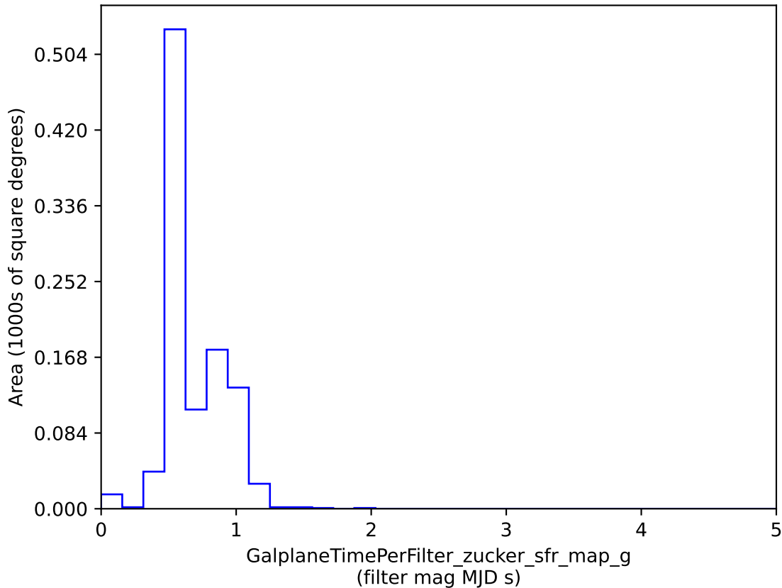
retro_baseline_v2.0_10yrs : GalplaneTimePerFilter_zucker_sfr_map_g
