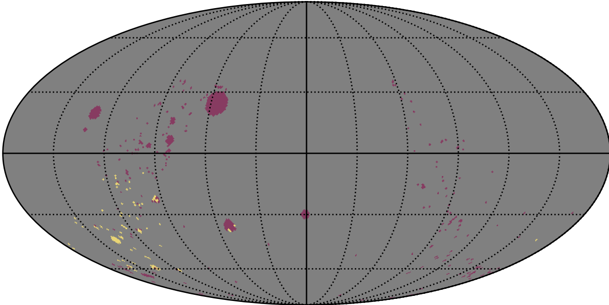
retro_baseline_v2.0_10yrs : GalplaneFootprintMetric_open_clusters_map_Tau_5_0
