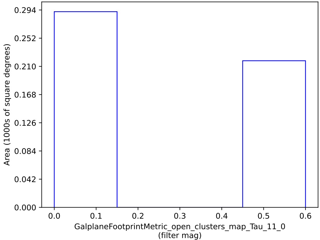
retro_baseline_v2.0_10yrs : GalplaneFootprintMetric_open_clusters_map_Tau_11_0
