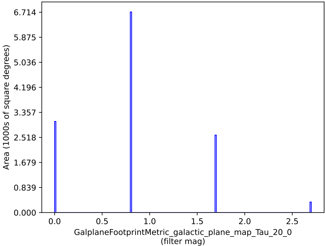
retro_baseline_v2.0_10yrs : GalplaneFootprintMetric_galactic_plane_map_Tau_20_0
