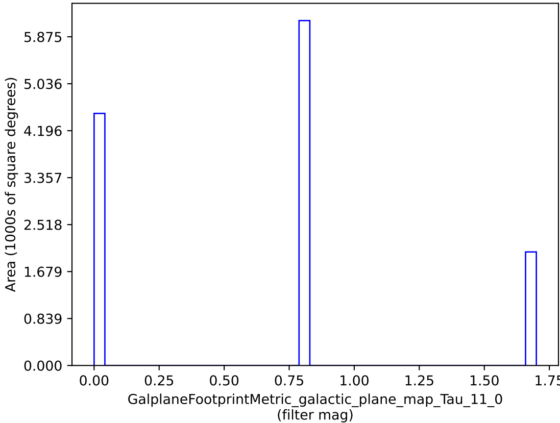
retro_baseline_v2.0_10yrs : GalplaneFootprintMetric_galactic_plane_map_Tau_11_0
