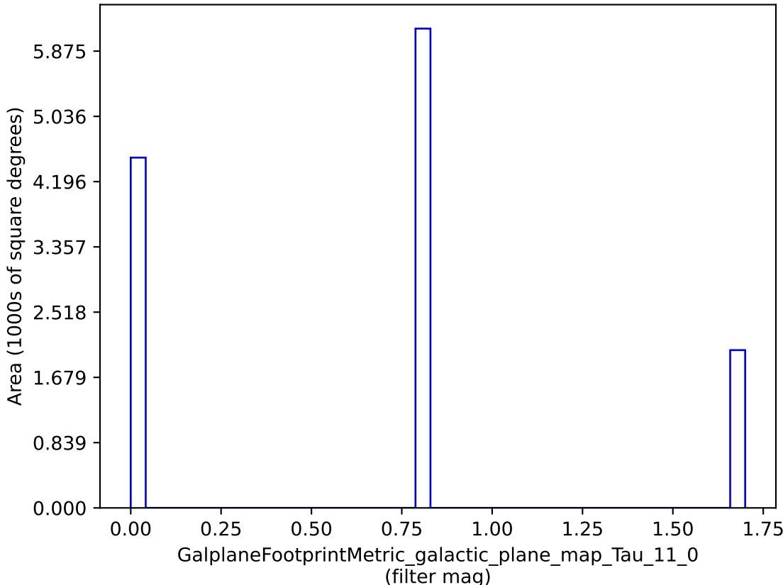
retro_baseline_v2.0_10yrs : GalplaneFootprintMetric_galactic_plane_map_Tau_11_0
