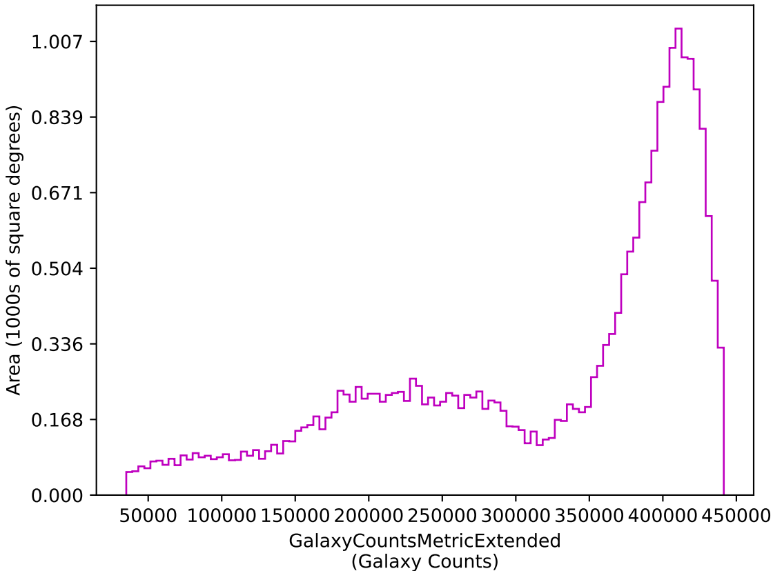
retro_baseline_v2.0_10yrs z: GalaxyCountsMetricExtended
