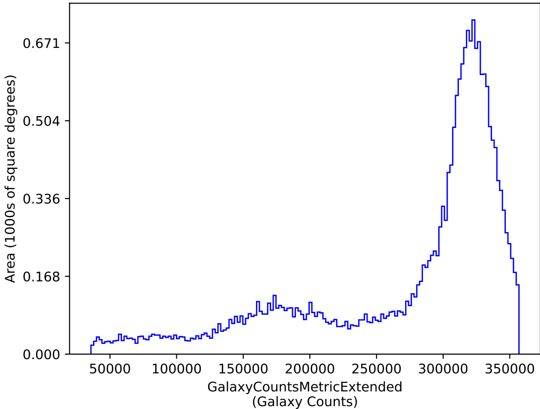
retro_baseline_v2.0_10yrs y: GalaxyCountsMetricExtended
