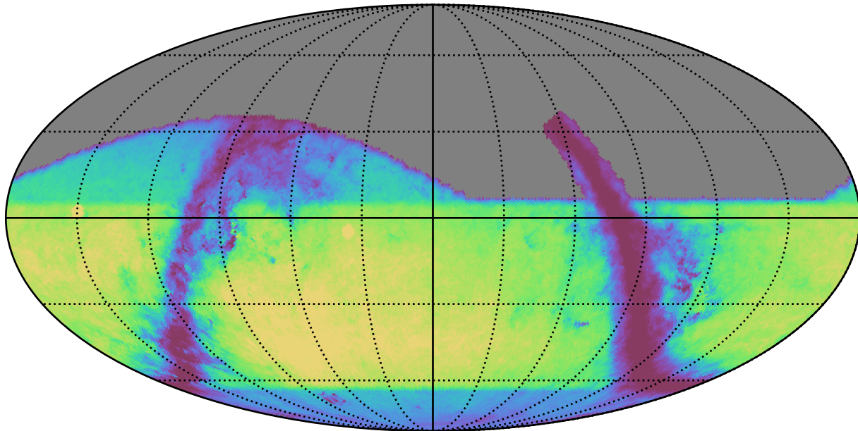
retro_baseline_v2.0_10yrs r: GalaxyCountsMetricExtended
