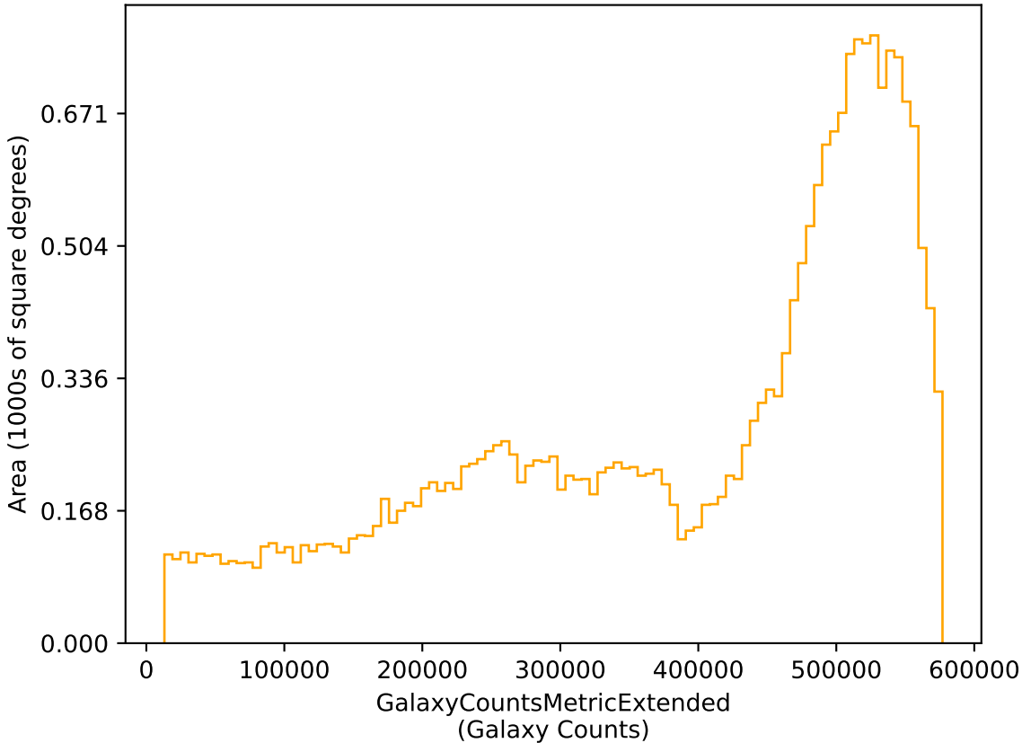
retro_baseline_v2.0_10yrs r: GalaxyCountsMetricExtended
