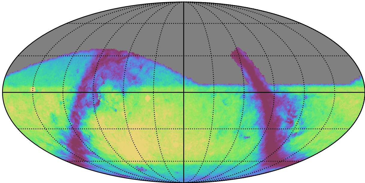
retro_baseline_v2.0_10yrs g: GalaxyCountsMetricExtended
