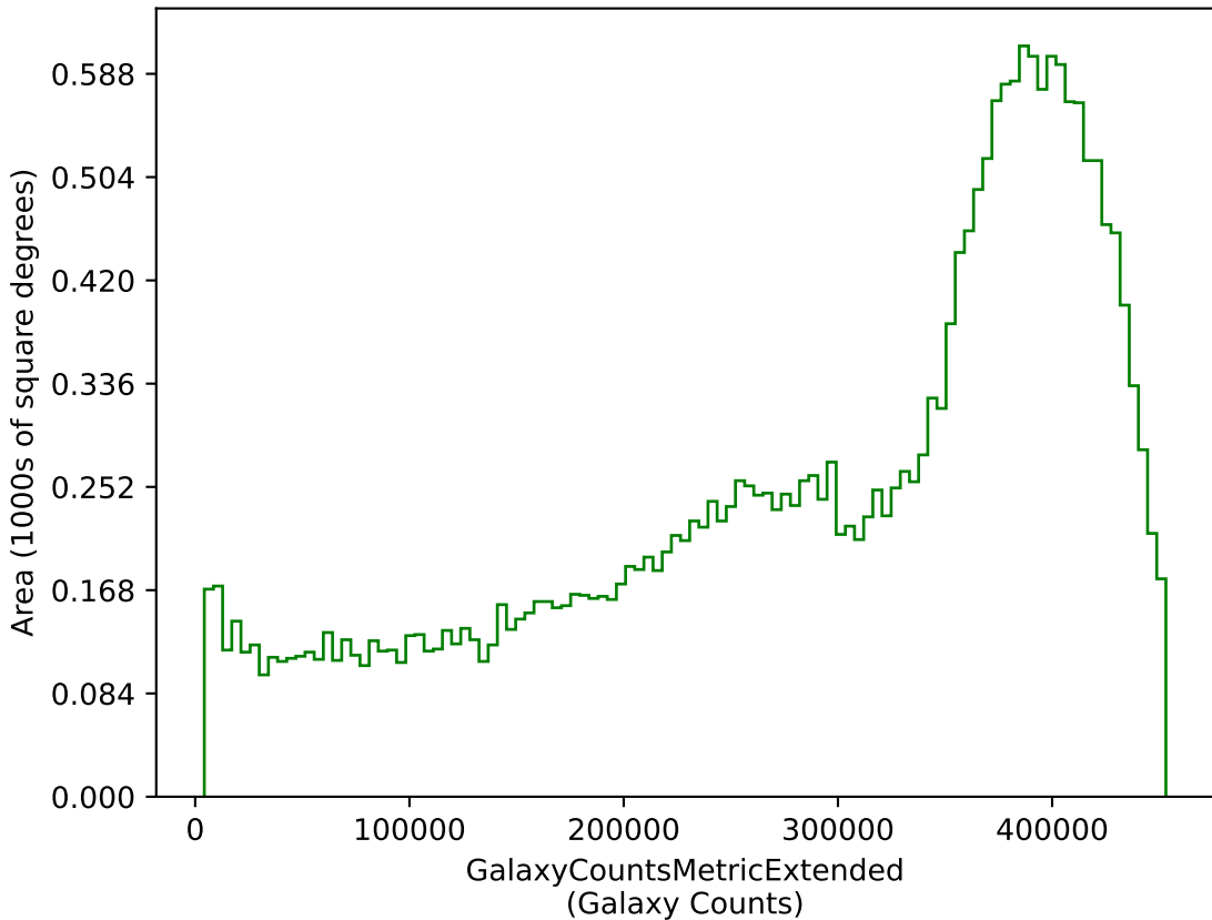
retro_baseline_v2.0_10yrs g: GalaxyCountsMetricExtended
