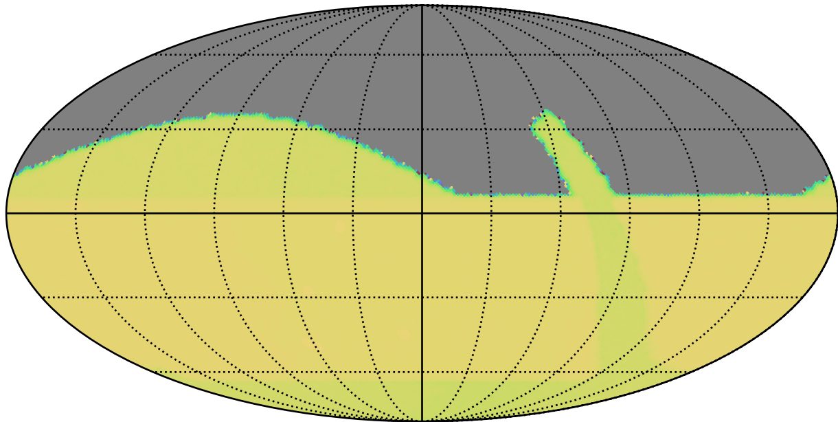
retro_baseline_v2.0_10yrs : GalPlaneVisitIntervalsTimescales_xray_binaries_map_Tau_46_5
