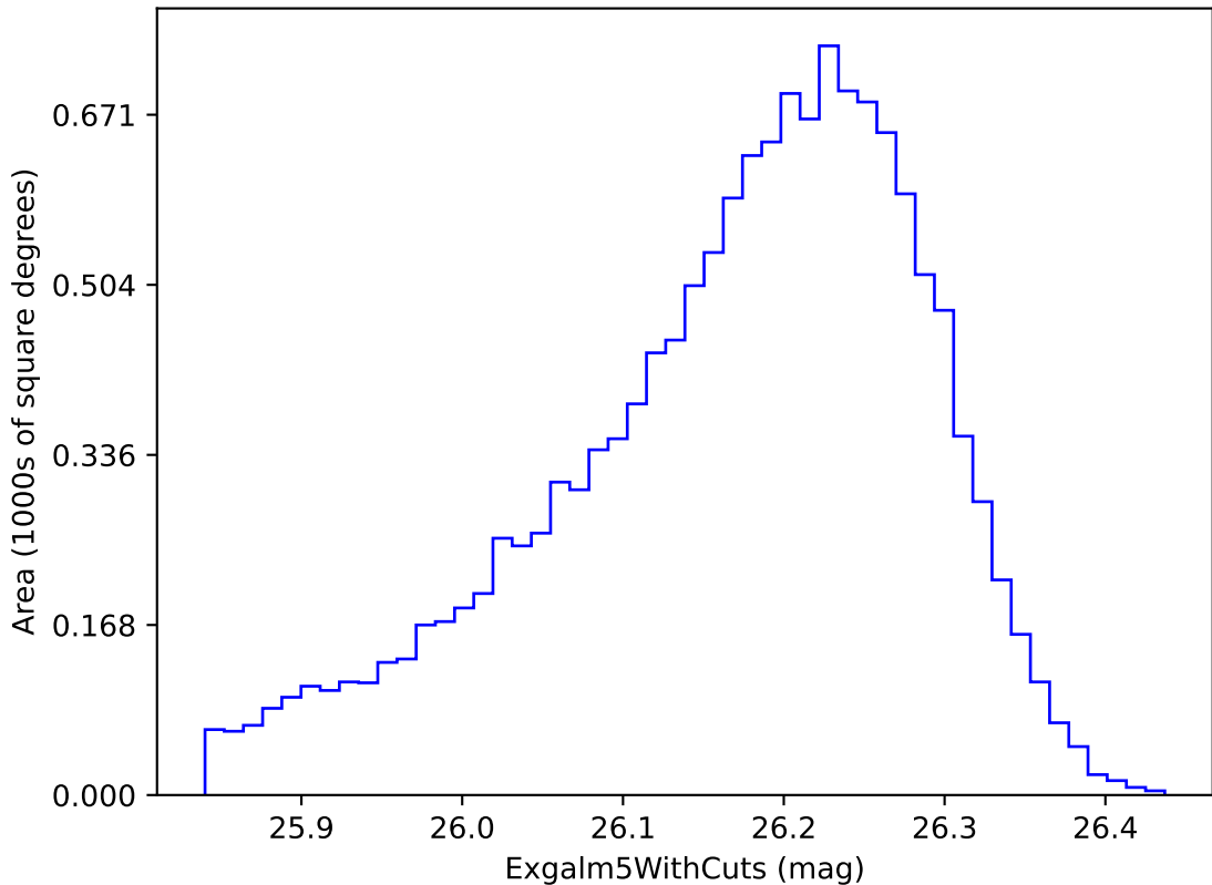
retro_baseline_v2.0_10yrs i band non-DD year 9: Exgalml5WithCuts
