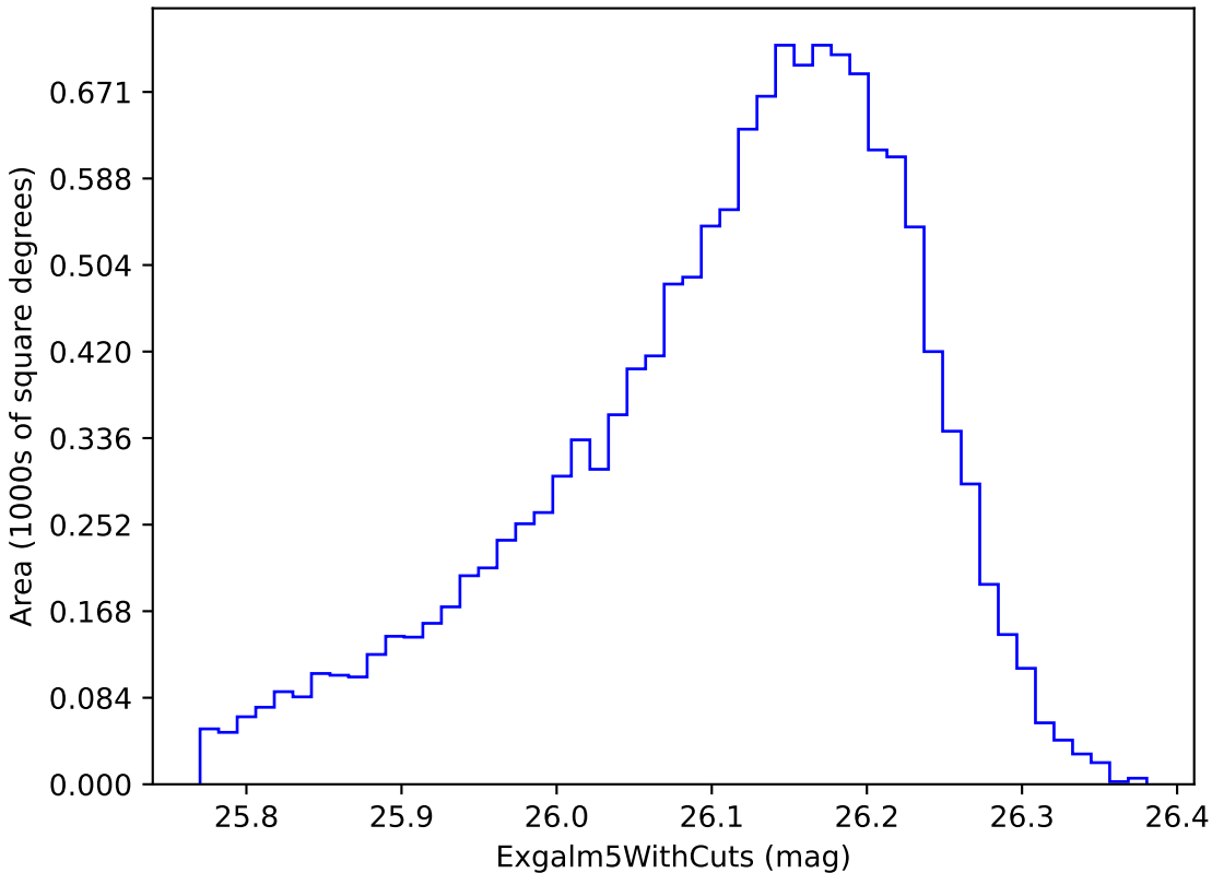
retro_baseline_v2.0_10yrs i band non-DD year 8: ExgalM5WithCuts
