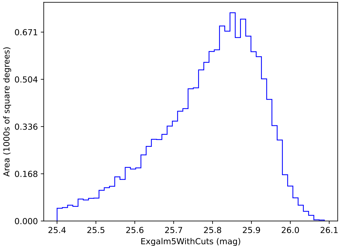
retro_baseline_v2.0_10yrs i band non-DD year 4: Exgalml5WithCuts
