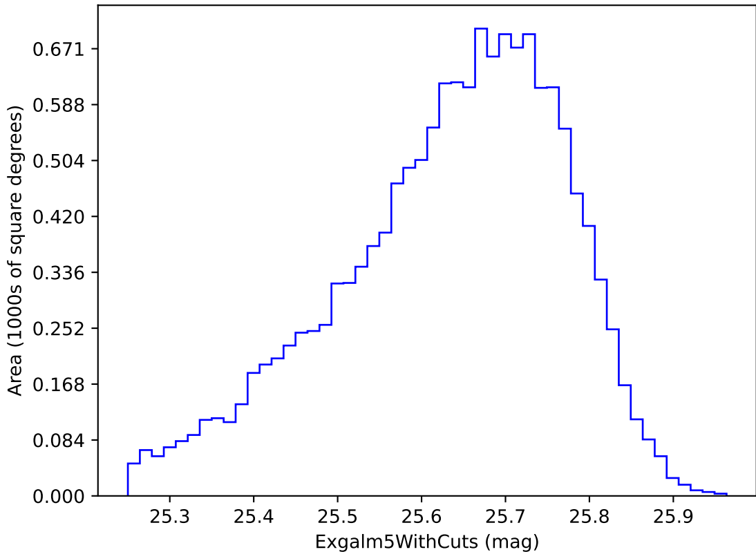
retro_baseline_v2.0_10yrs i band non-DD year 3: ExgalM5WithCuts
