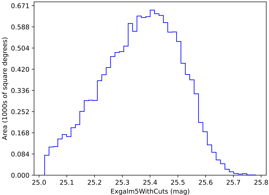
retro_baseline_v2.0_10yrs i band non-DD year 2: ExgalM5WithCuts
