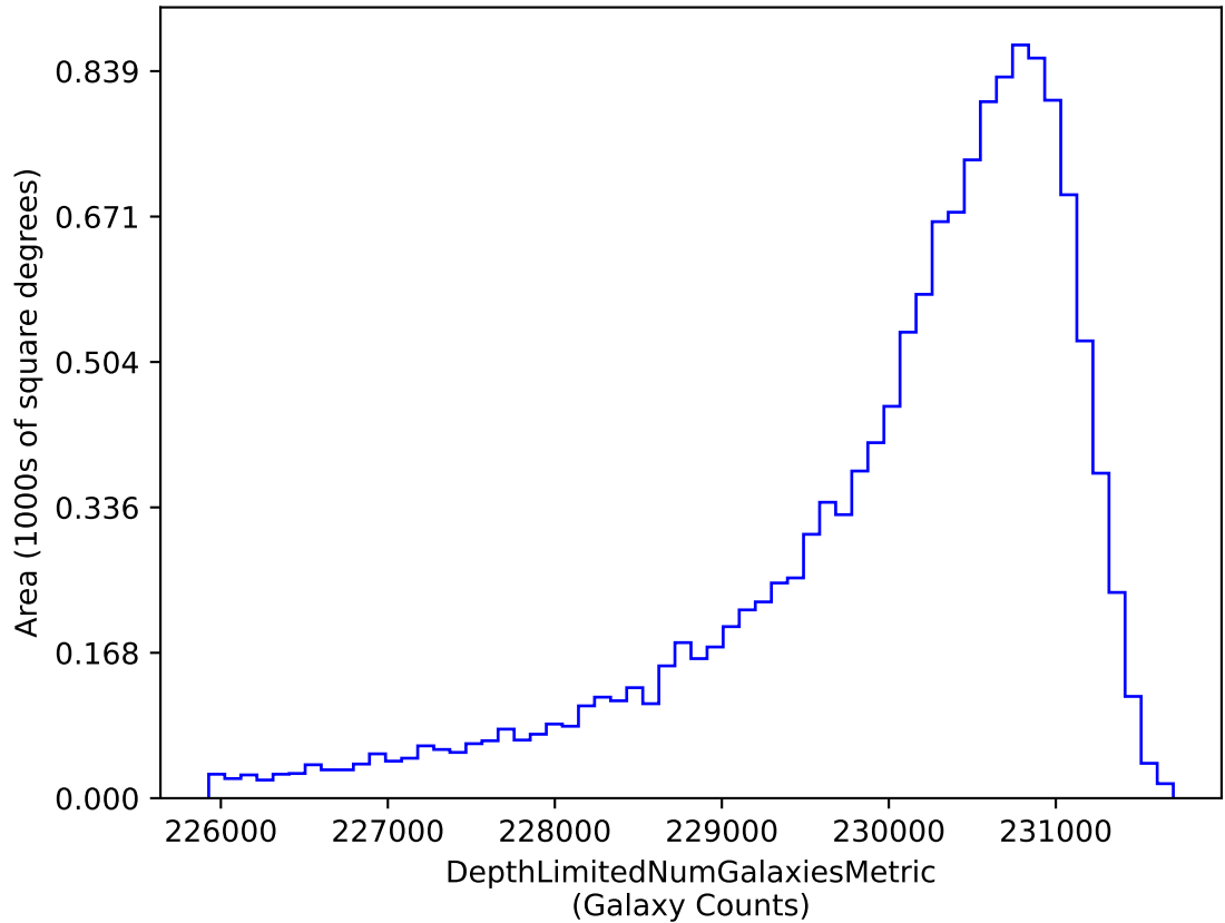
retro_baseline_v2.0_10yrs i band galaxies non-DD: DepthLimitedNumGalaxiesMetric
