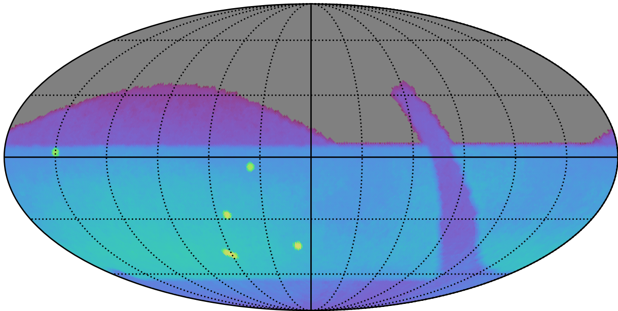
retro_baseline_v2.0_10yrs : Brown Dwarf, L7
