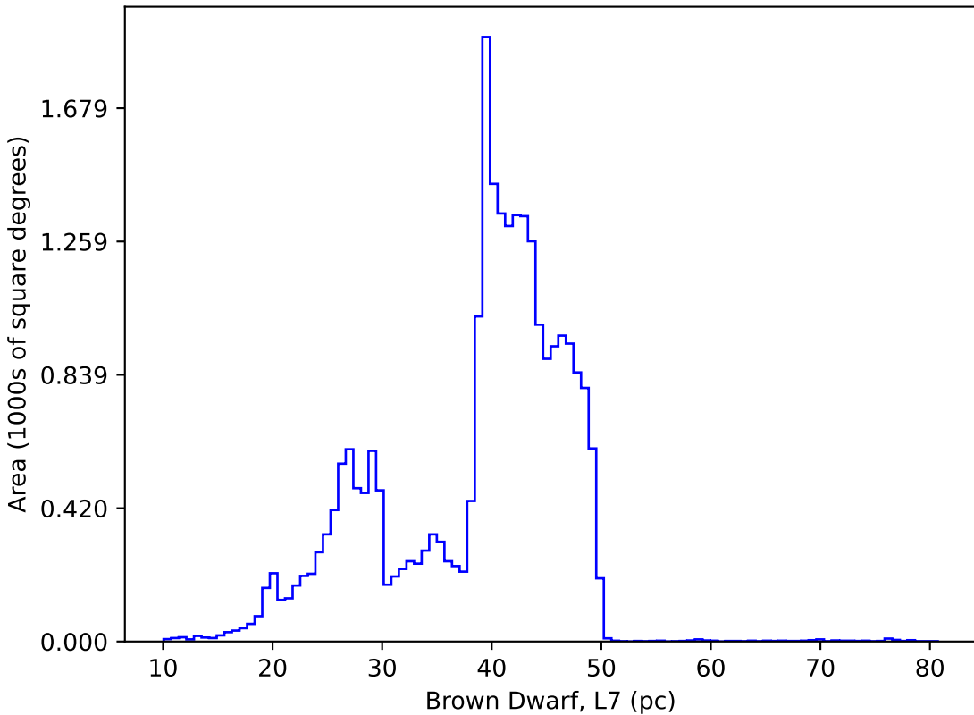
retro_baseline_v2.0_10yrs : Brown Dwarf, L7
