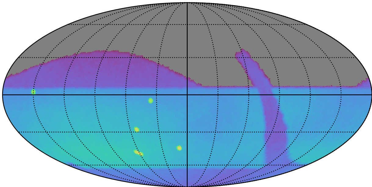
retro_baseline_v2.0_10yrs : Brown Dwarf, L4
