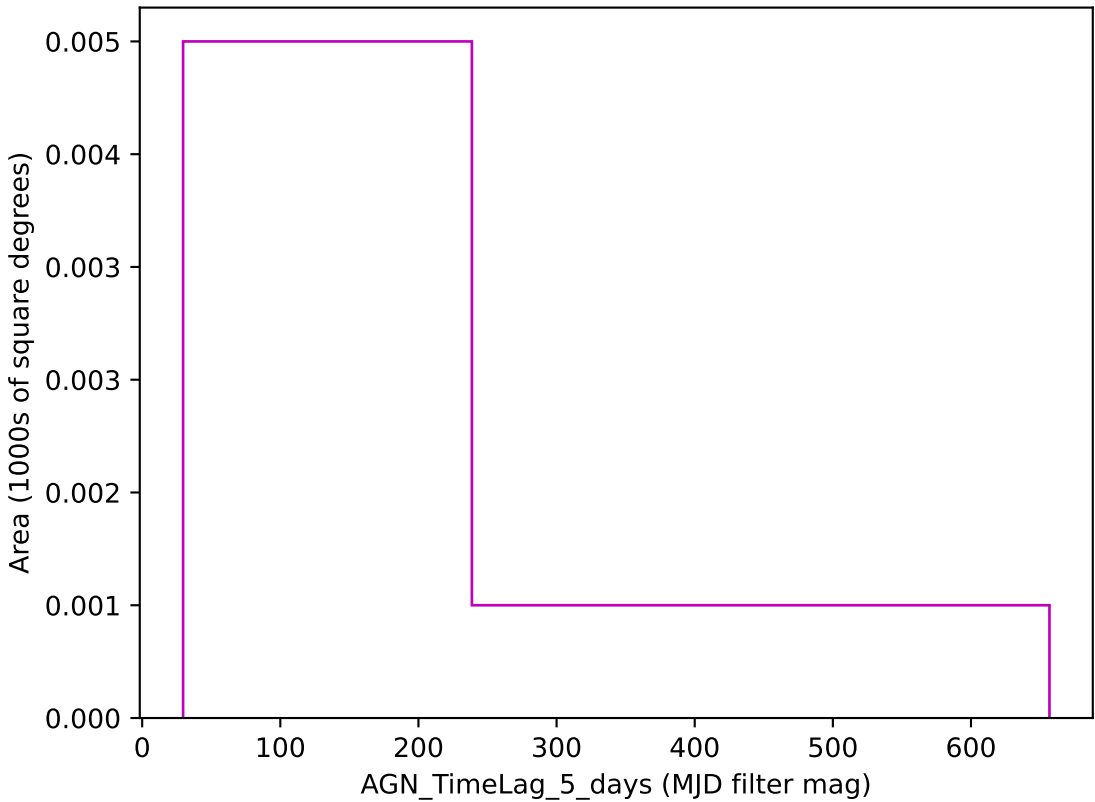
retro_baseline_v2.0_10yrs z band: AGN_TimeLag_5_days
