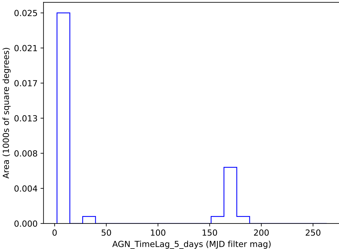
retro_baseline_v2.0_10yrs y band: AGN_TimeLag_5_days
