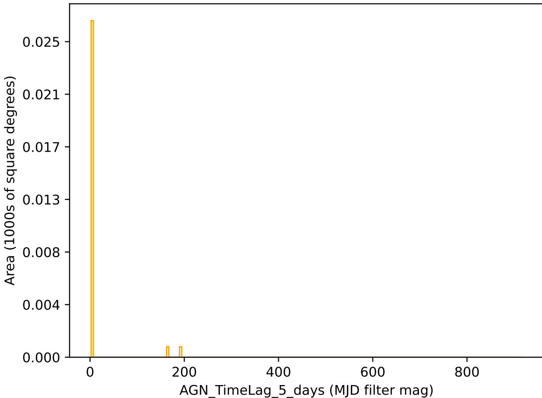
retro_baseline_v2.0_10yrs r band: AGN_TimeLag_5_days
