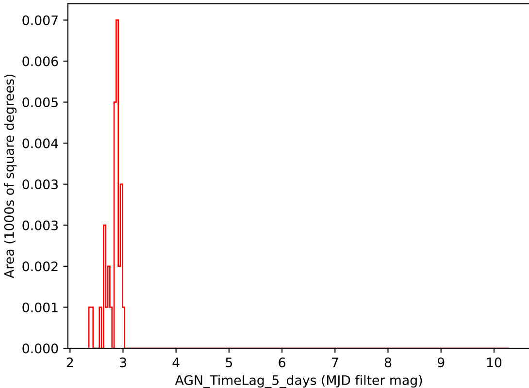
retro_baseline_v2.0_10yrs i band: AGN_TimeLag_5_days
