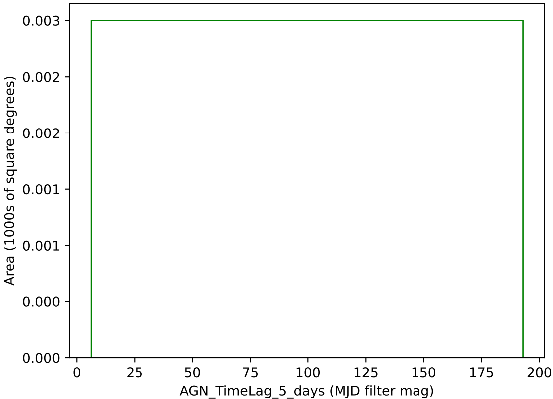
retro_baseline_v2.0_10yrs g band: AGN_TimeLag_5_days
