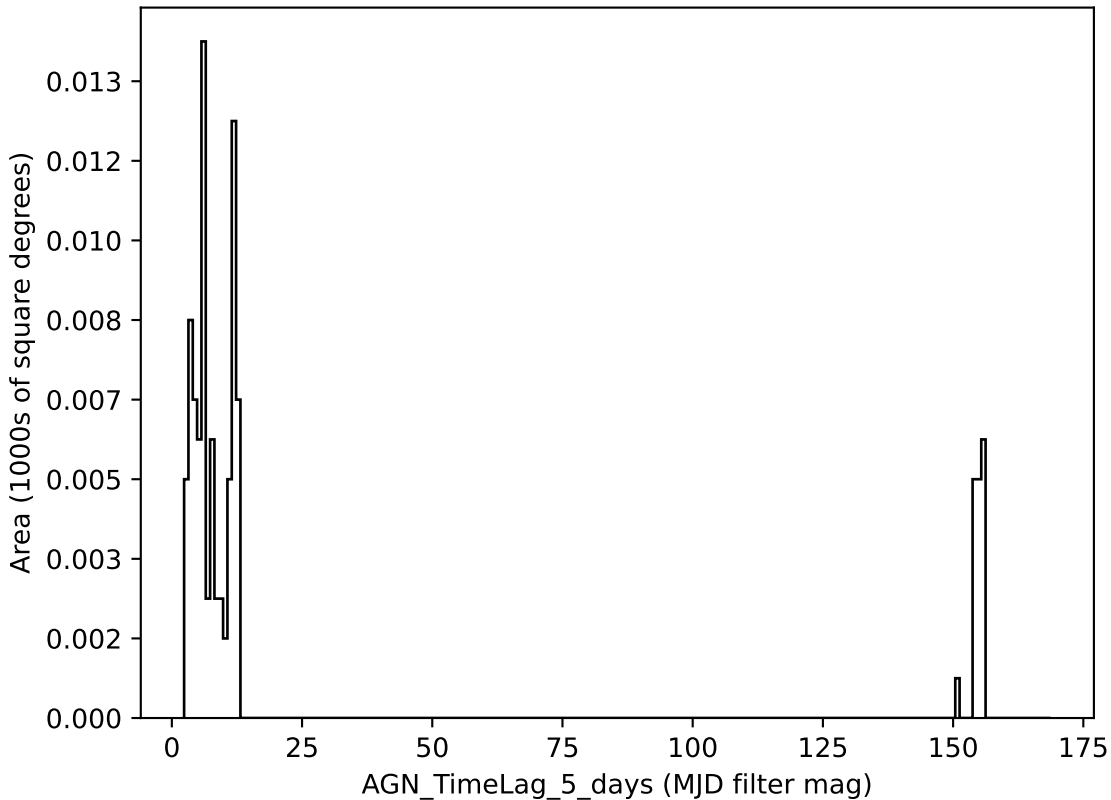
retro_baseline_v2.0_10yrs all bands: AGN_TimeLag_5_days
