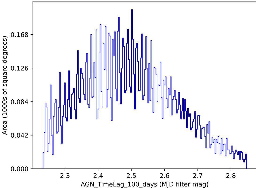
retro_baseline_v2.0_10yrs y band: AGN_TimeLag_100_days
