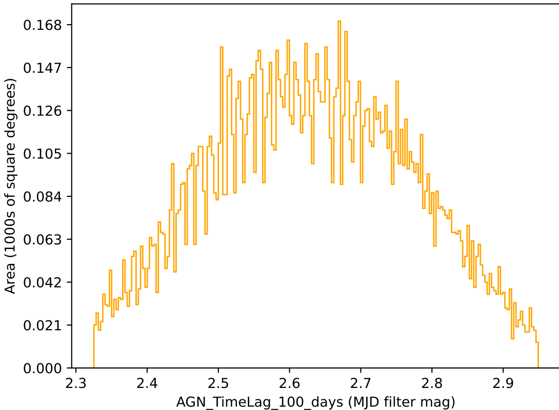
retro_baseline_v2.0_10yrs r band: AGN_TimeLag_100_days
