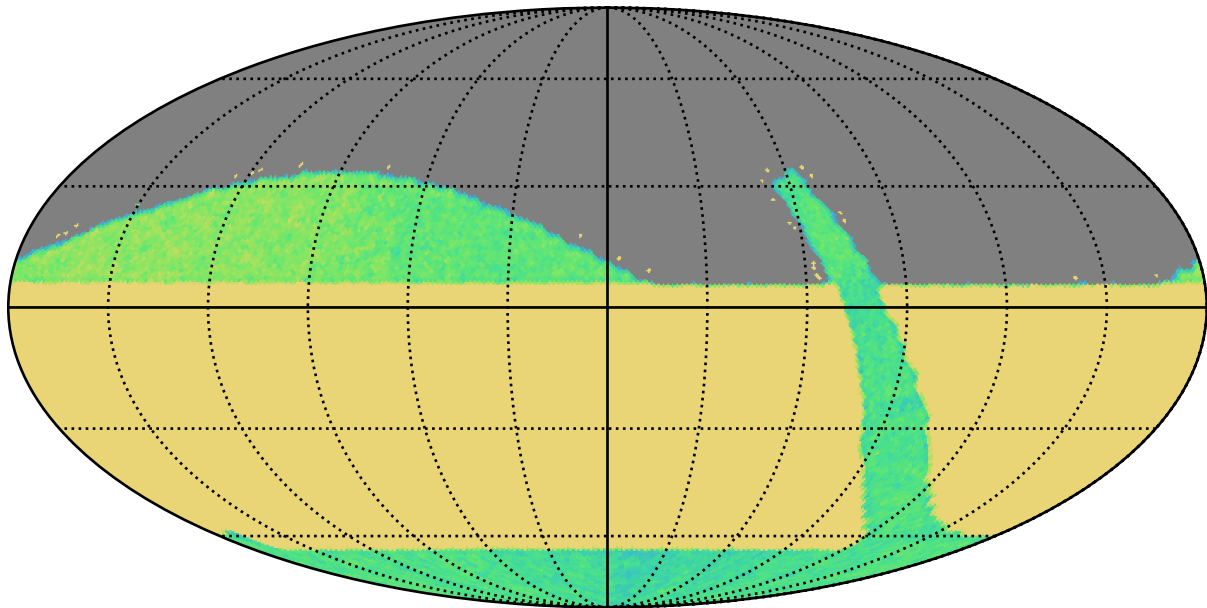
retro_baseline_v2.0_10yrs all bands: AGN_TimeLag_100_days
