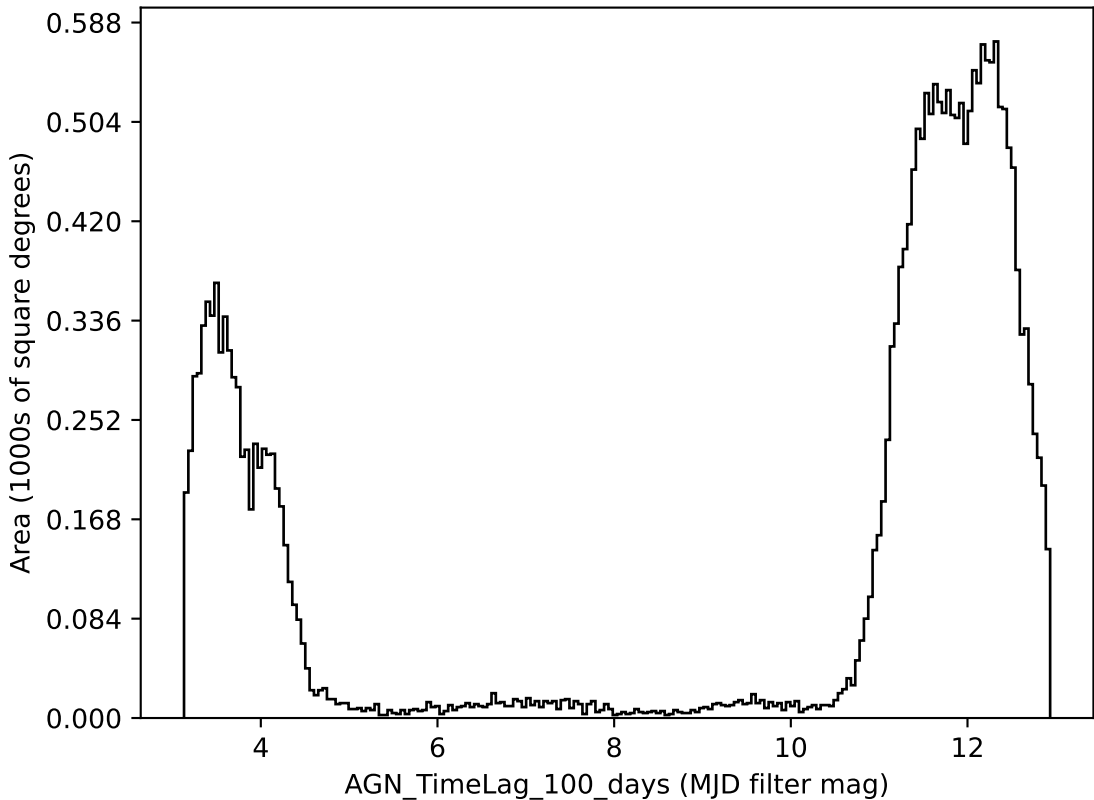
retro_baseline_v2.0_10yrs all bands: AGN_TimeLag_100_days
