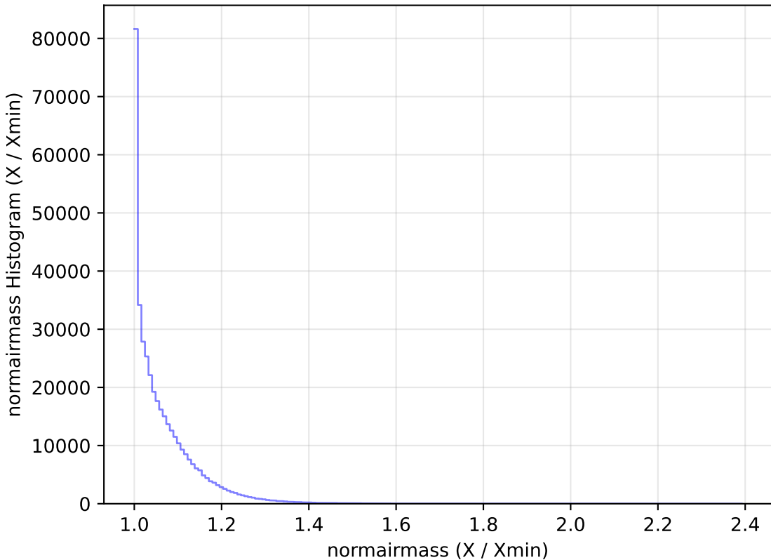
retro_baseline_v2.0_10yrs WFD z band: normairmass Histogram
