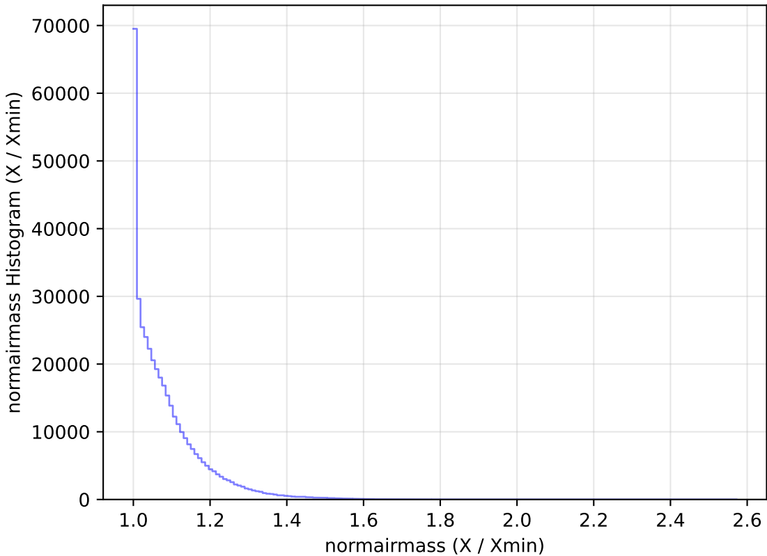
retro_baseline_v2.0_10yrs WFD y band: normairmass Histogram
