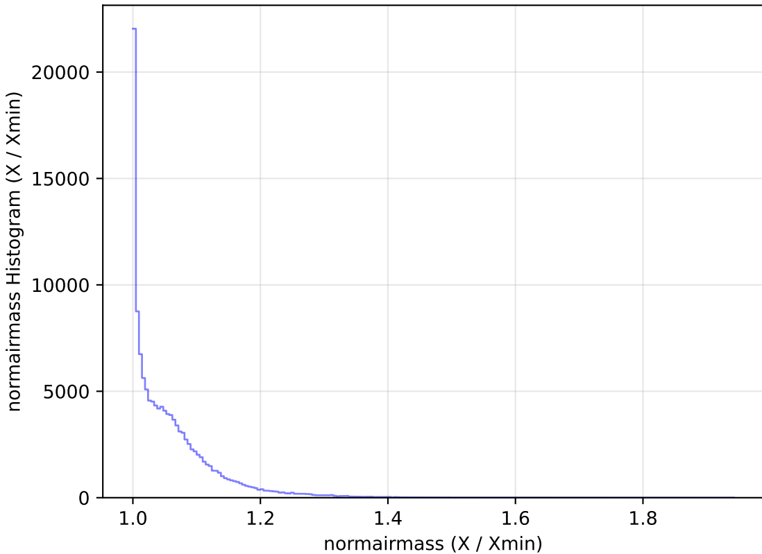
retro_baseline_v2.0_10yrs WFD u band: normairmass Histogram
