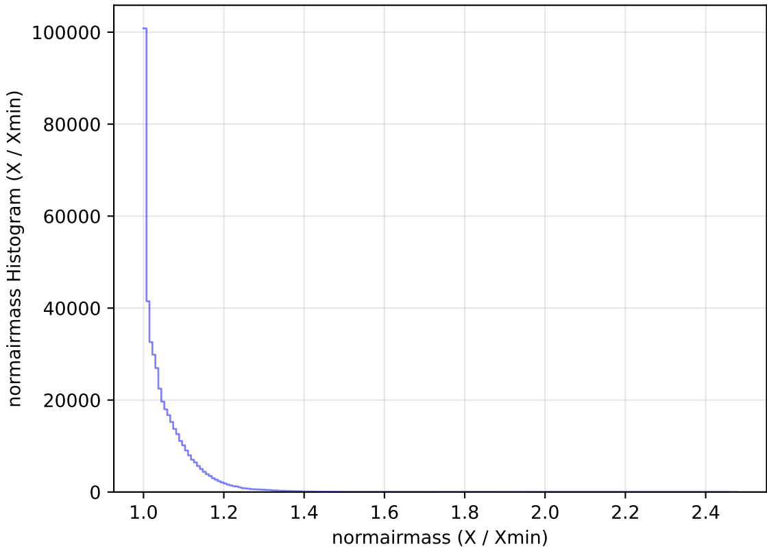
retro_baseline_v2.0_10yrs WFD r band: normairmass Histogram
