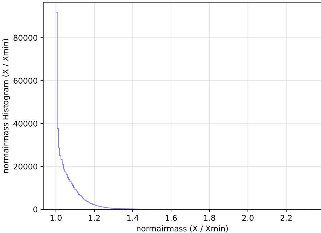
retro_baseline_v2.0_10yrs WFD i band: normairmass Histogram
