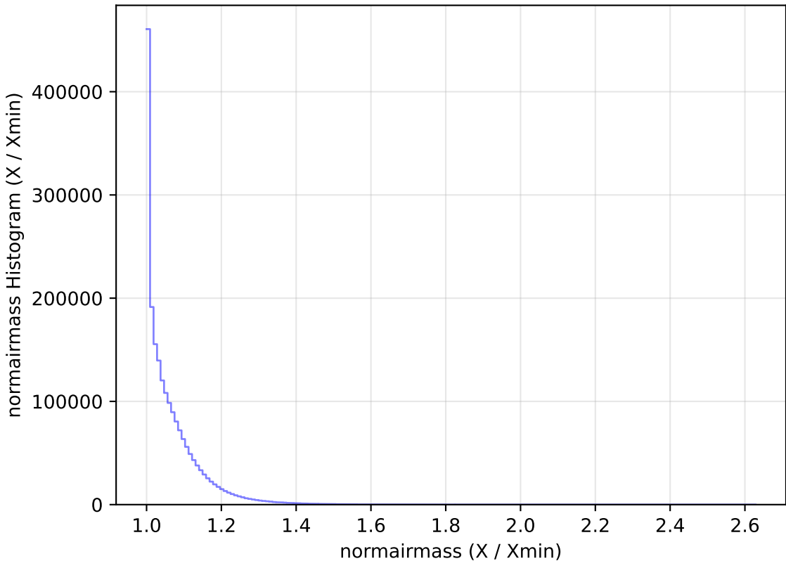
retro_baseline_v2.0_10yrs WFD all bands: normairmass Histogram
