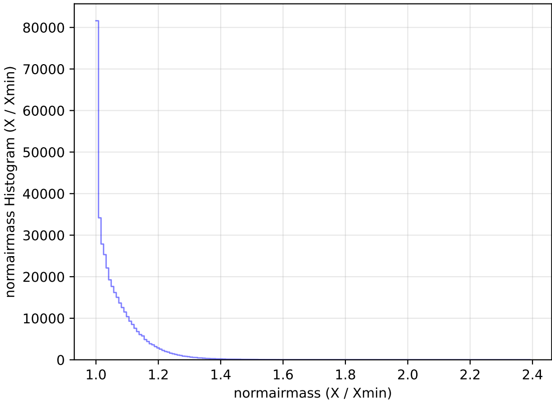
retro_baseline_v2.0_10yrs All sky z band: normairmass Histogram
