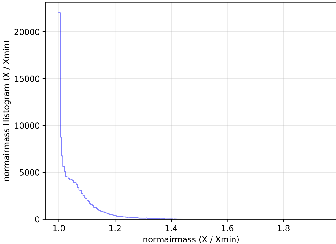
retro_baseline_v2.0_10yrs All sky u band: normairmass Histogram
