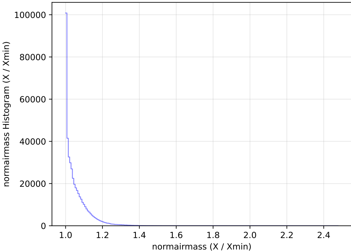
retro_baseline_v2.0_10yrs All sky r band: normairmass Histogram
