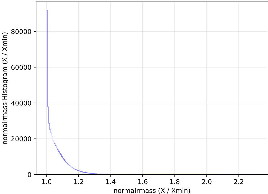
retro_baseline_v2.0_10yrs All sky i band: normairmass Histogram
