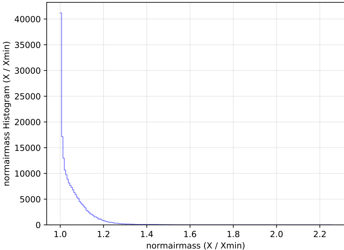
retro_baseline_v2.0_10yrs All sky g band: normairmass Histogram
