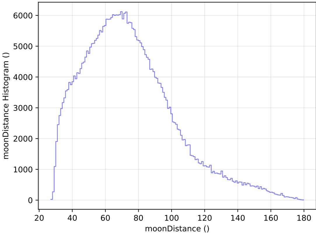
retro_baseline_v2.0_10yrs WFD z band: moonDistance Histogram
