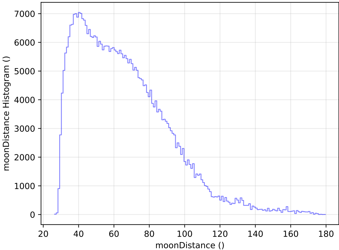
retro_baseline_v2.0_10yrs WFD y band: moonDistance Histogram
